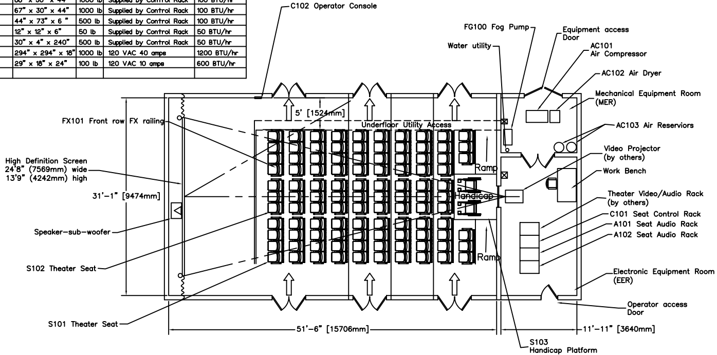
THEATER PLAN Scale 1:50
