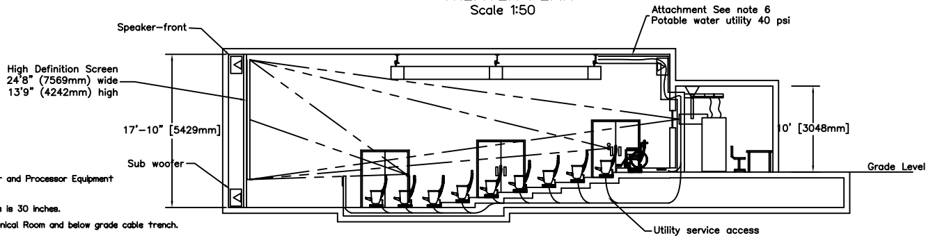
THEATER SECTION Scale 1:50
